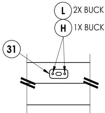
DETAIL 1 Attach astragal throw bolt strike plate to frame as shown
