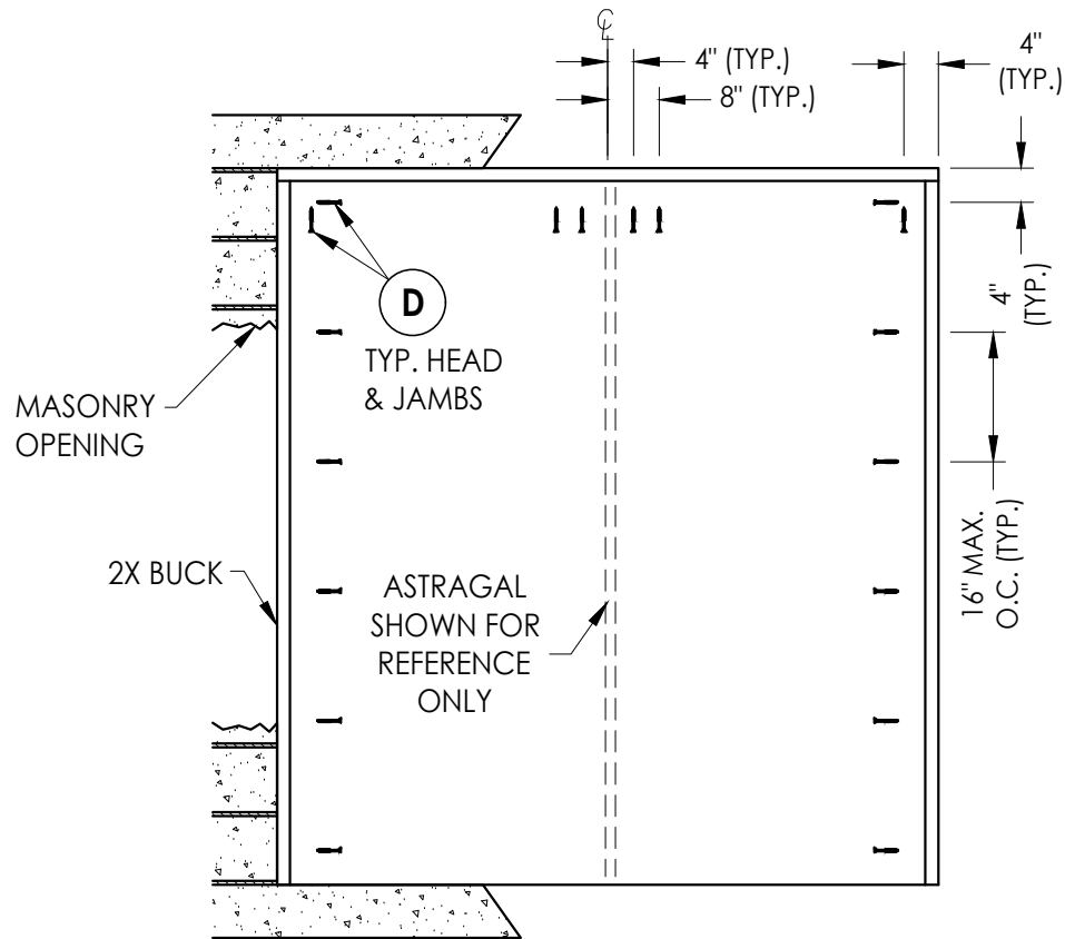
BUCK ANCHORING XX
